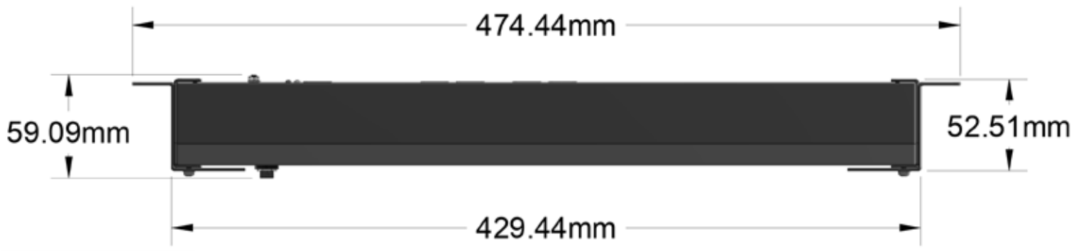
Optional DIN rail mounted version
